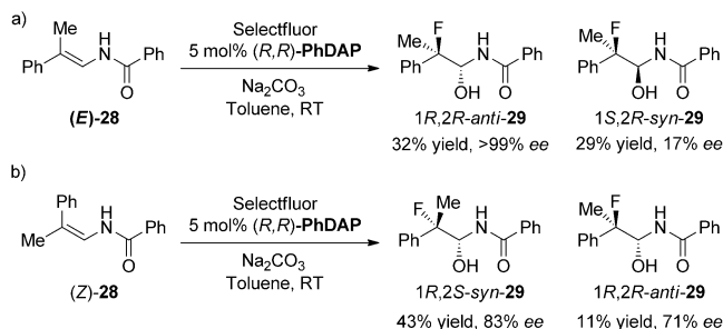
Scheme 2. Double stereodifferentiation in the formation of a quaternary fluorine stereocenter. Relative and absolute configuration of syn -29 determined by X-ray crystallography (see the Supporting Information for details). All other products assigned by tentative analogy.
