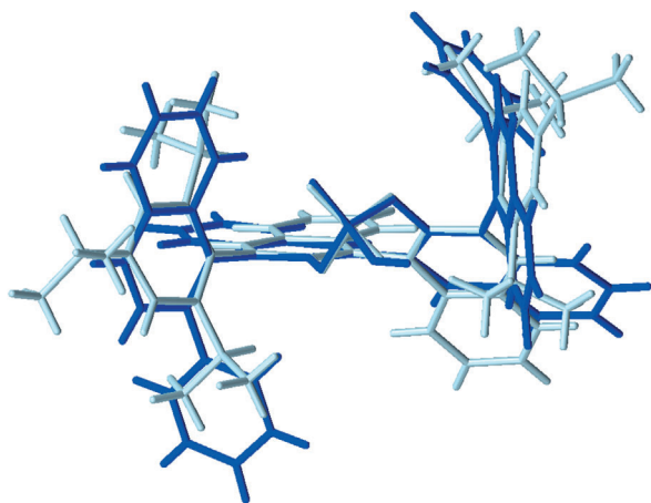
Figure 1. Overlay of X-ray crystal structures of TRIP (cyan) and PhDAP (blue).
