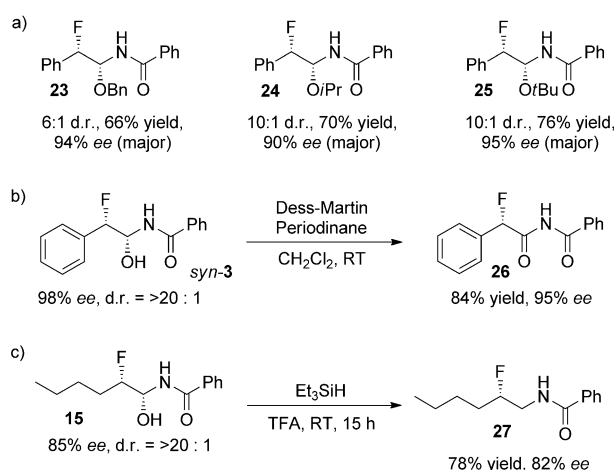
Scheme 1. Fluoroalkoxylation and elaboration of products. Yields refer to yields of isolated syn and anti diastereomers. See the Supporting Information for reaction conditions.
